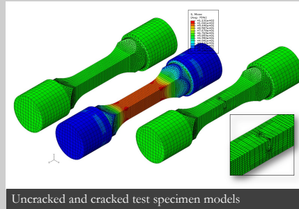
Uncracked and cracked test specimen models
