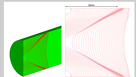
Calculated profiles: corner and through crack phases
