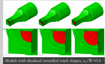
Models with idealised tunnelled crack shapes, a_0/W=0.4
