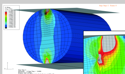
Von Mises stress for a model with a single defect
