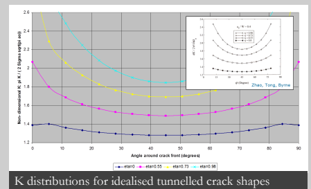
K distributions for idealised tunnelled crack shapes
