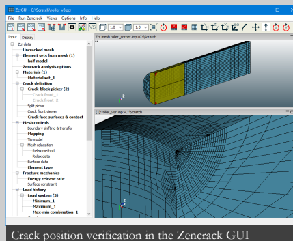
Crack position verification in the Zencrack GUI
