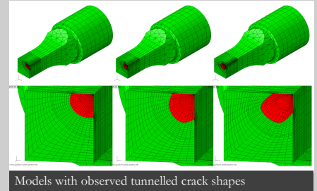
Models with observed tunnelled crack shapes
